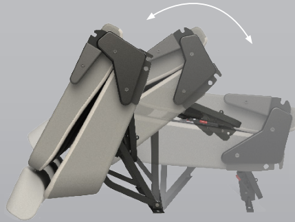
Release leg catch to fold forward and pull front pins to remove seat.
